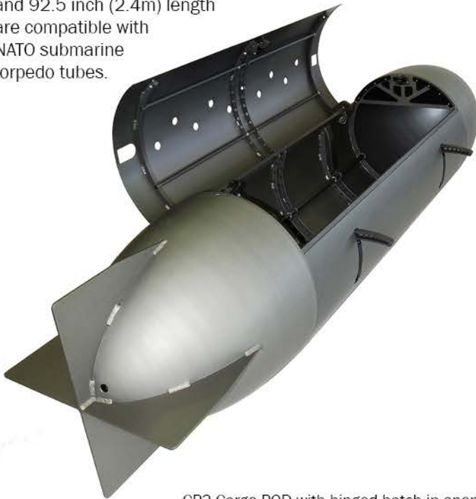
CP3 Cargo POD with hinged hatch in open position
