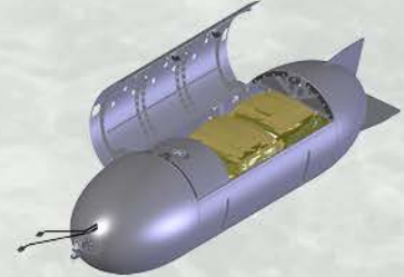
LB190 Long Single Battery Shallow Water PowerPOD
