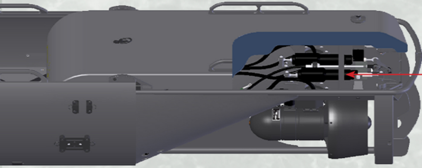
View of AC3 exposing installed RNAV3 and AP3 actuators
